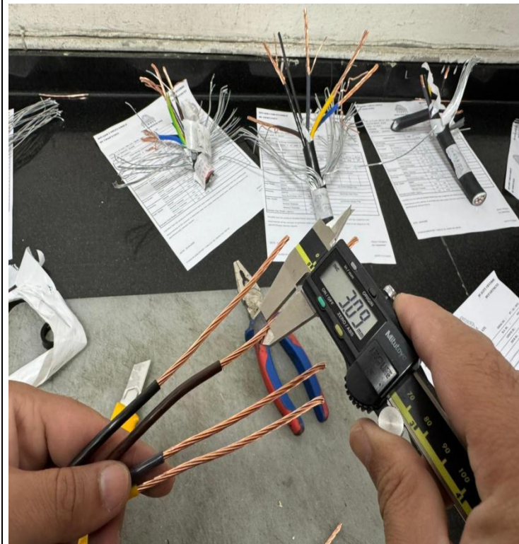
Diameter of the conductor
