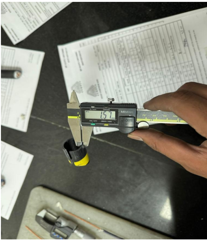
Thickness of Outer Sheath
