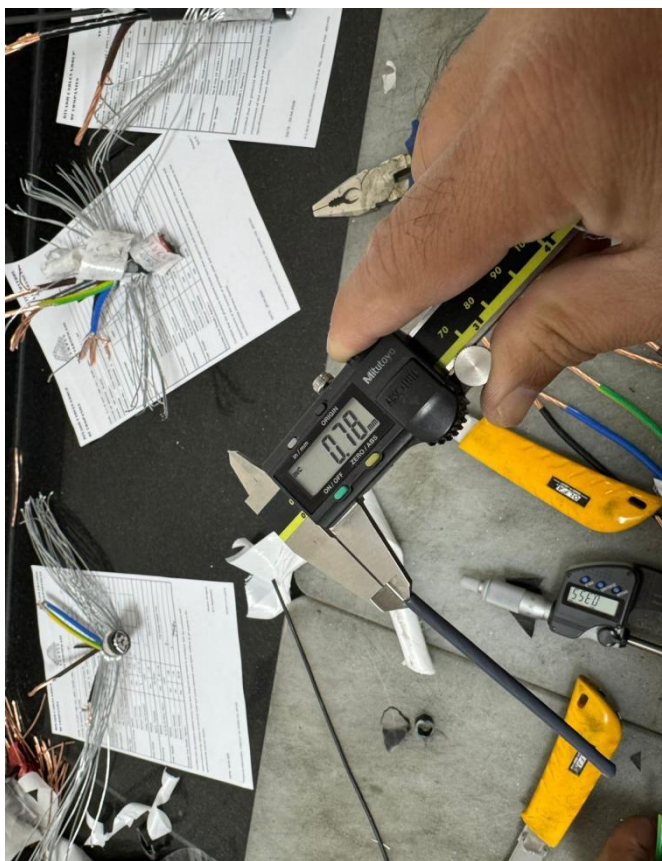
Thickness of XLPE Insulation
