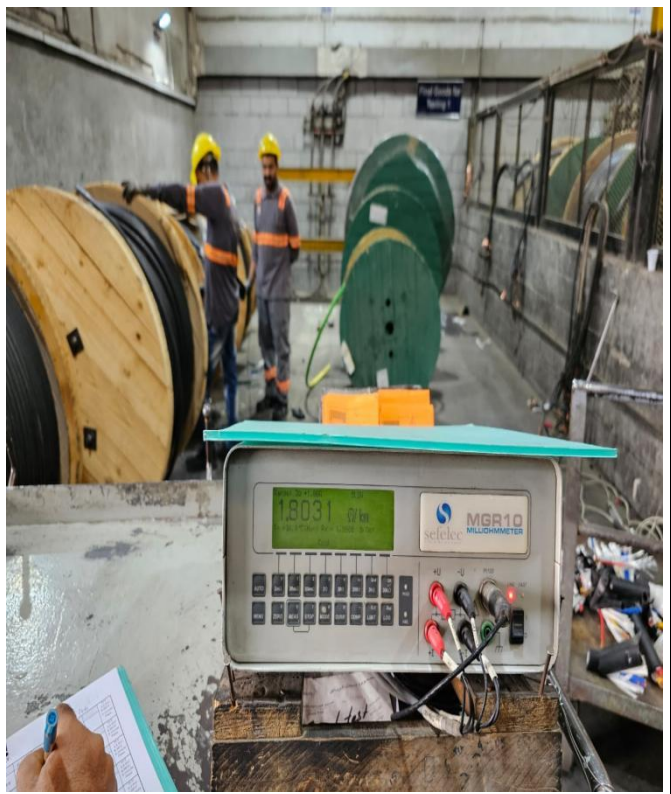
Conductor Resistance
