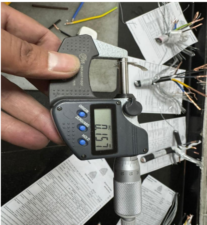
Thickness of mica tape
