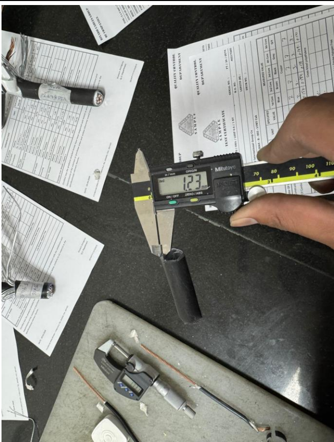
Thickness of Inner Sheath
